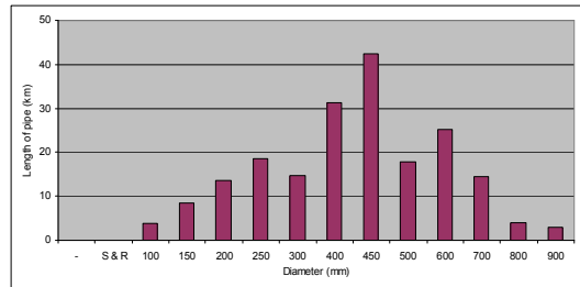
Length of each pipe diameter in the Baseline solution
